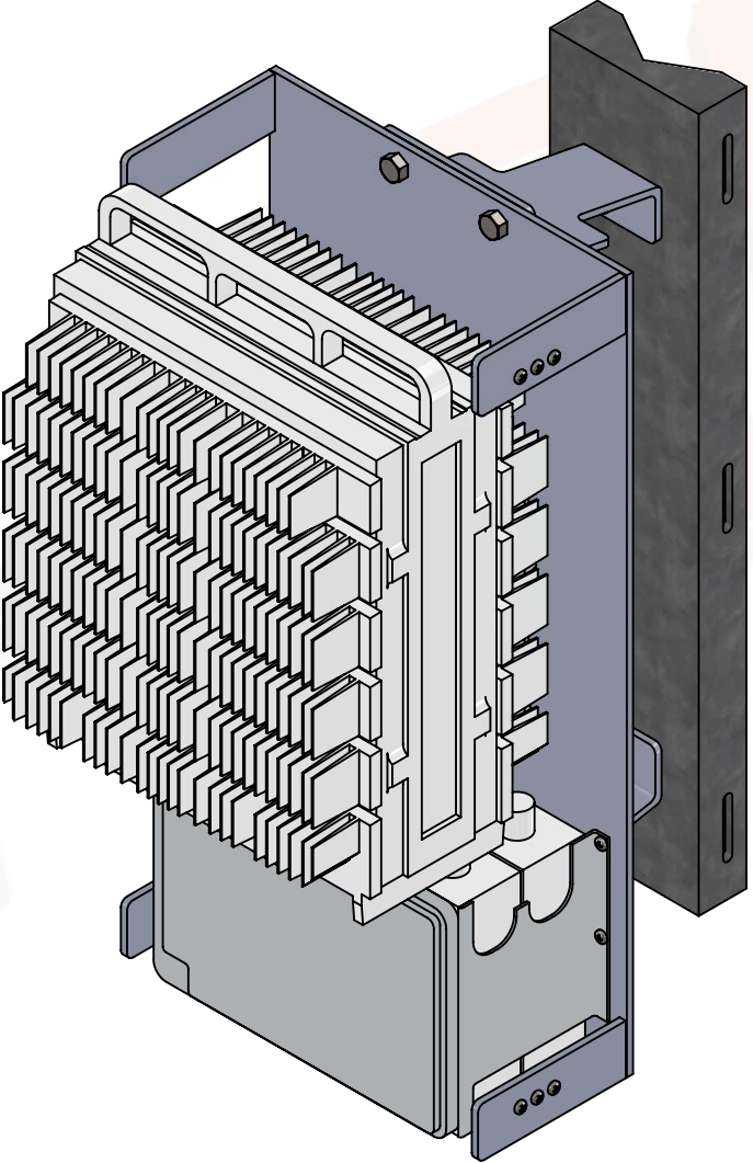
SHROUD REMOVED TO SHOW 8843 RADIO AND DIPLEXERS
